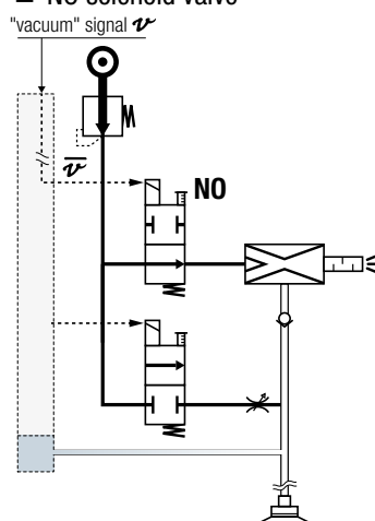
■ NO solenoid valve
