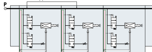
common pressure supplied to units
