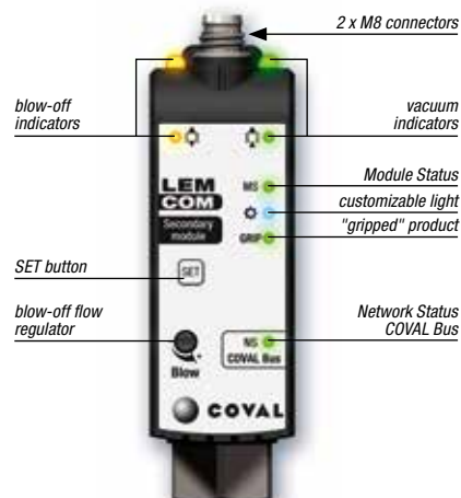
LEMCOM secondary module
