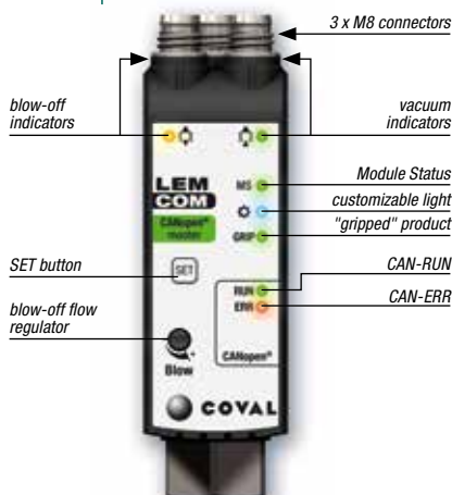
LEMCOM master CANopen
