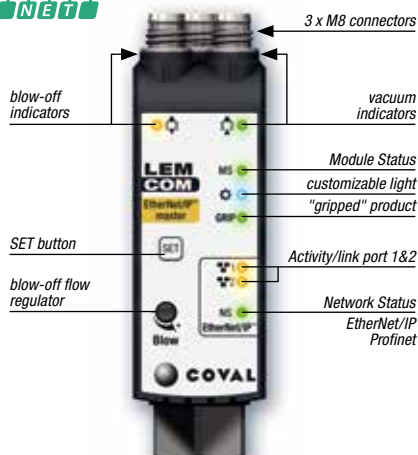
LEMCOM master PROFI EtherNet/IP
